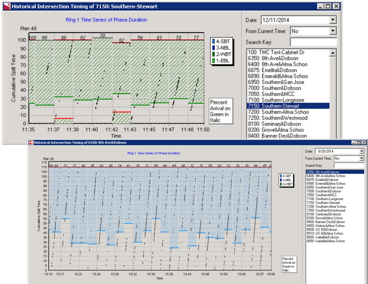
Purdue coordination diagrams showing percent arrivals on green for each cycle
